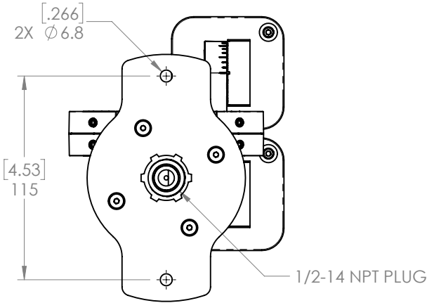
VIEW A-A (BOTTOM VIEW)
